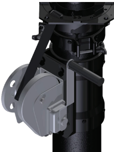
ST Series Tiger Winch P/N: ST-WINCH01
